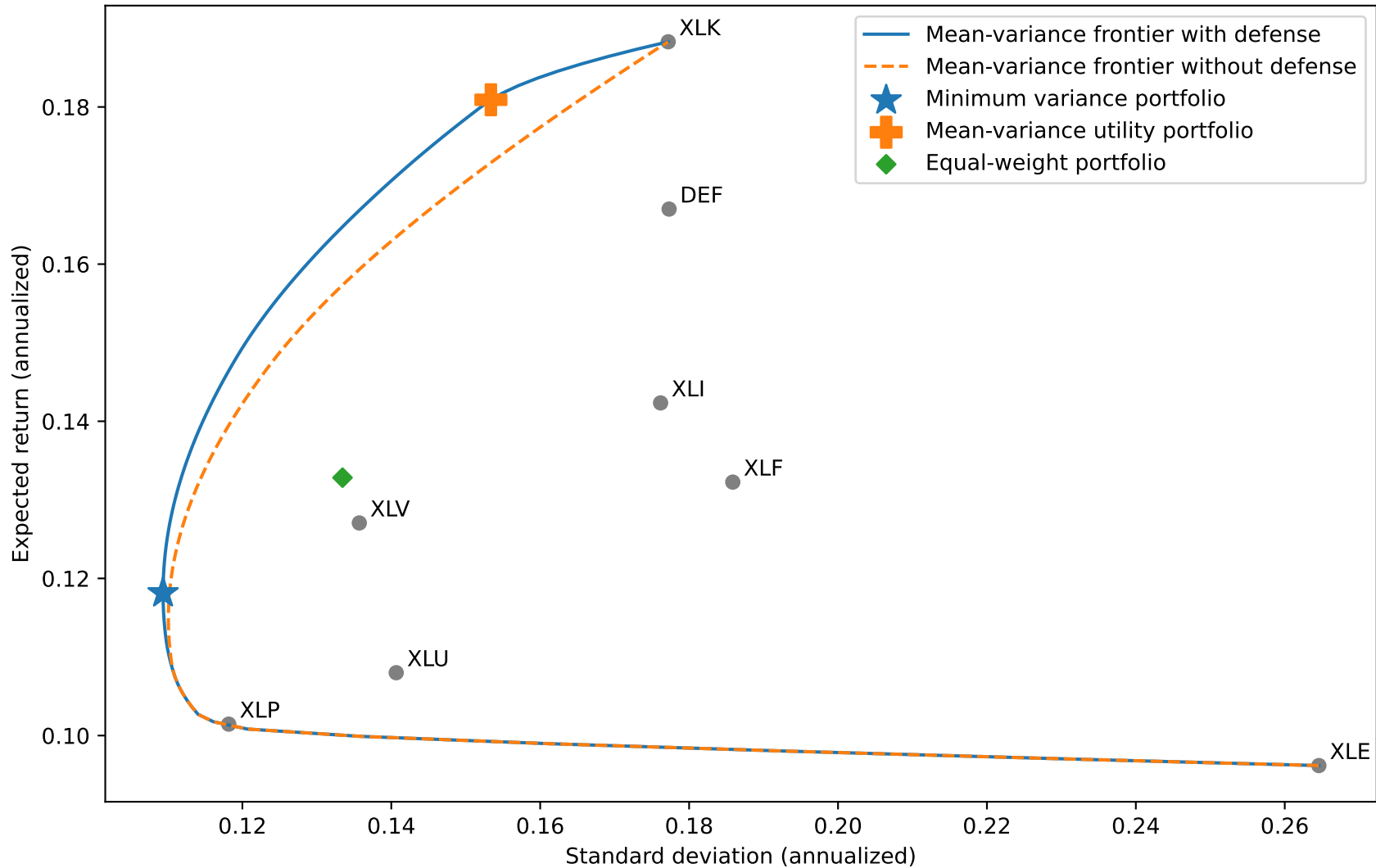
Mean-variance frontier, Jan 2010 to Dec 2025
